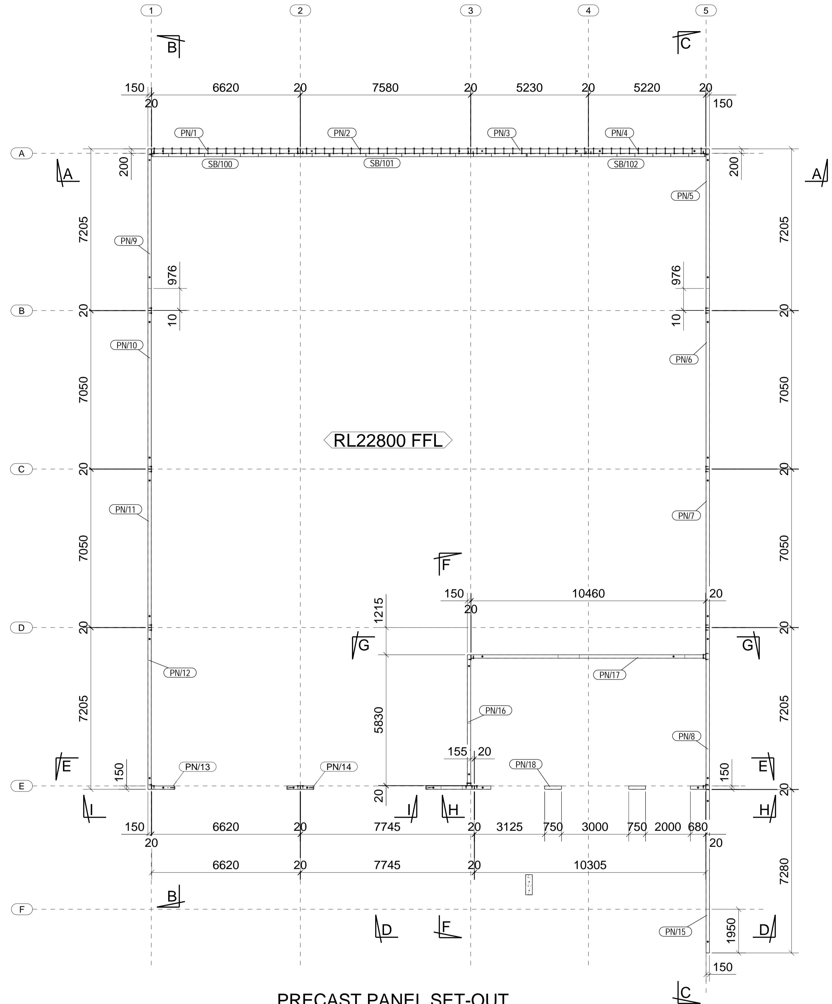
PRECAST PANEL SET-OUT
