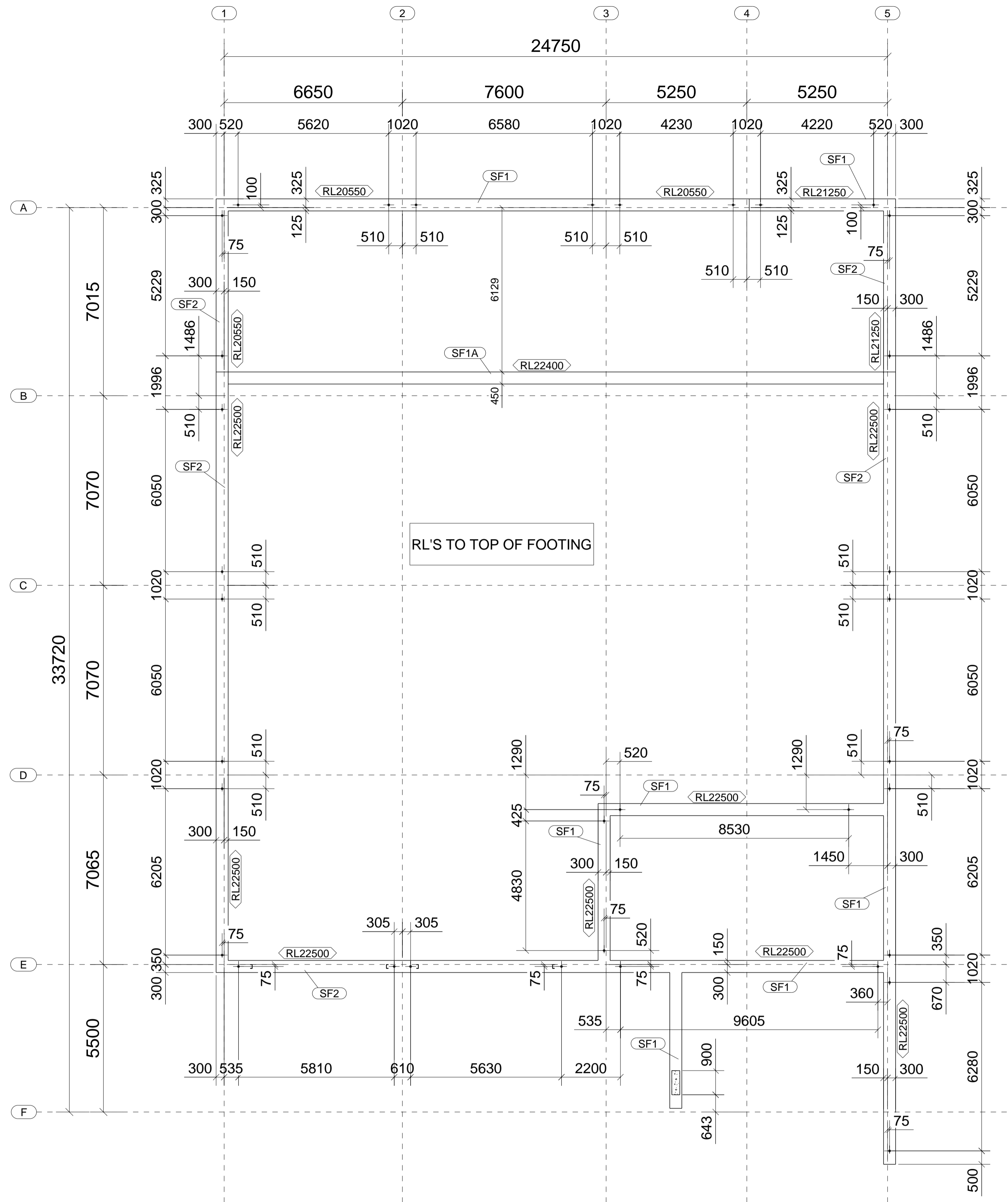
FOOTING LOCATING PIN SET-OUT
